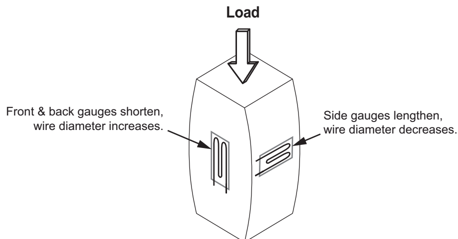
Figure 5-12. Strain Gauge
