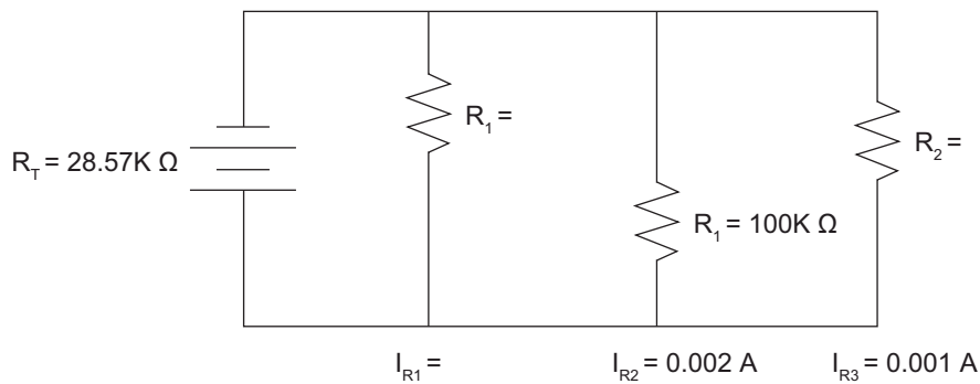
Figure 5-5. Parallel Resistive Circuit
