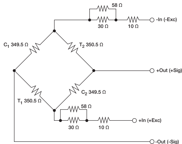
Figure 6-2. Wheatstone Bridge
